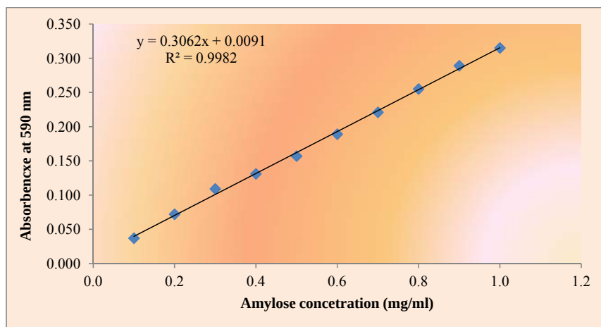
Fig. 2.3: Standard graph of amylose using iodine reagent
