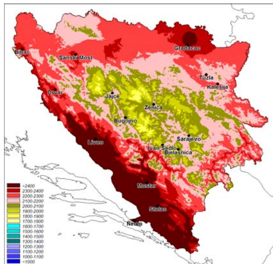
Figure 2. Spatial distribution of insolation (h) in 2017
