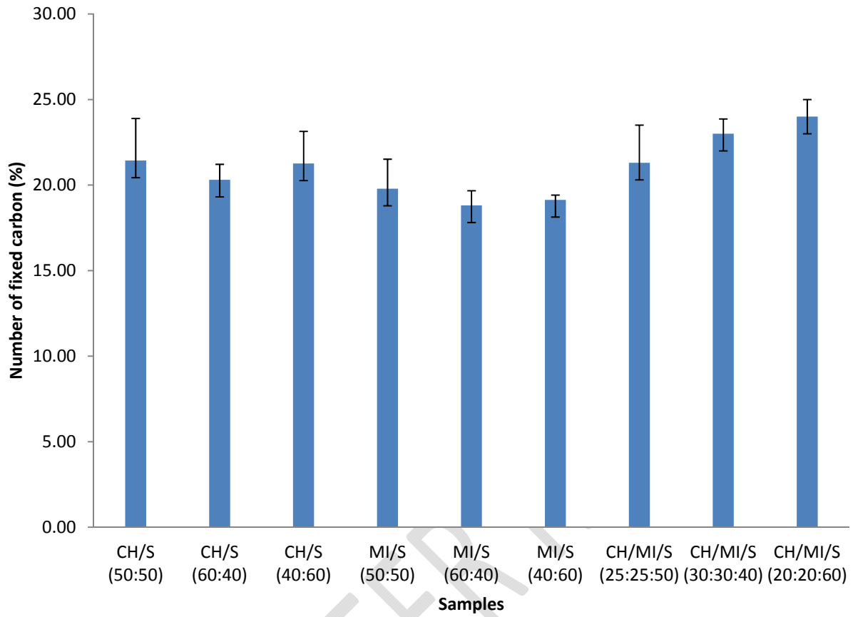
Fig. 3: Bar chart showing variations in the number of fixed carbon in of the samples
