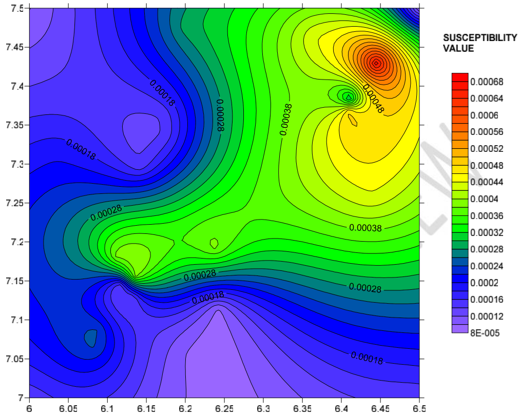
Fig.5. Magnetic Susceptibility map of the Study Area Showing Rock Contrasts
