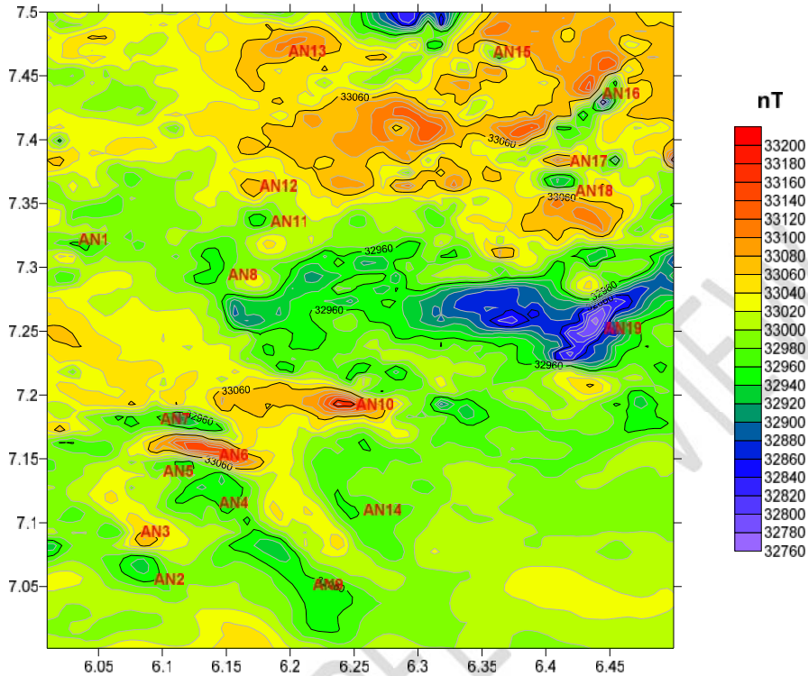
Fig.3. TMI map of Auchi sheet showing the Magnetic Intensity Values
