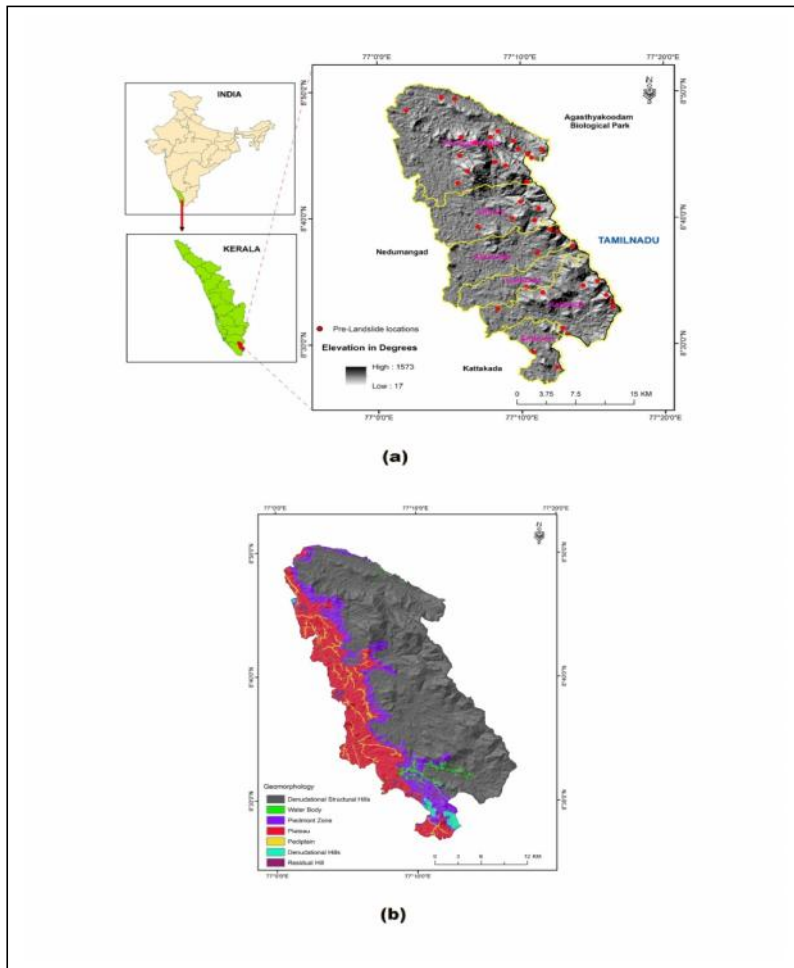
Fig :1 (a) Study Area(b) Geomorphology
