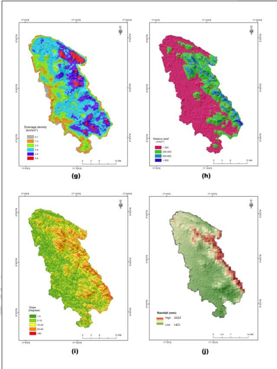
Fig: 3 (g) Drainage density (h) Relative relief (i) Slope (j) Rainfall
