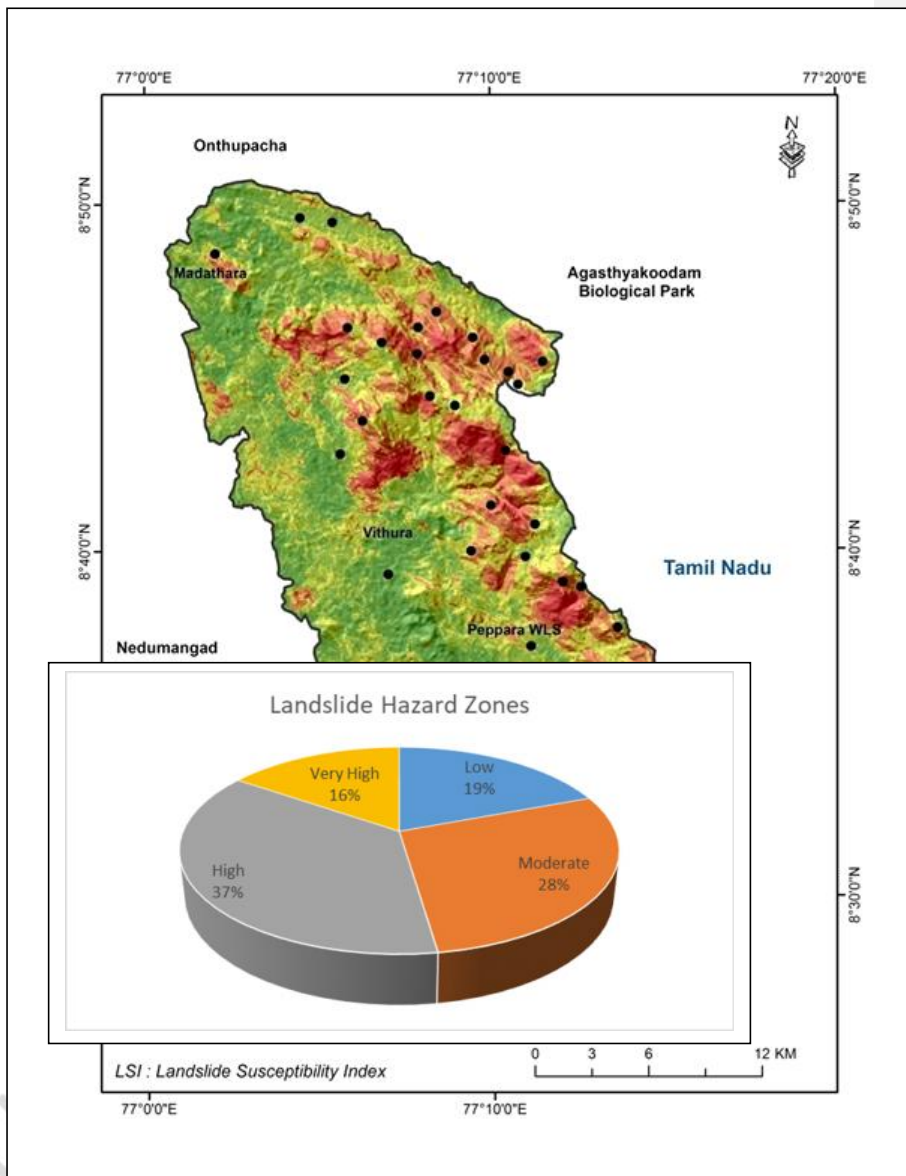
Fig: 4 Landslide Susceptibility Index Map
