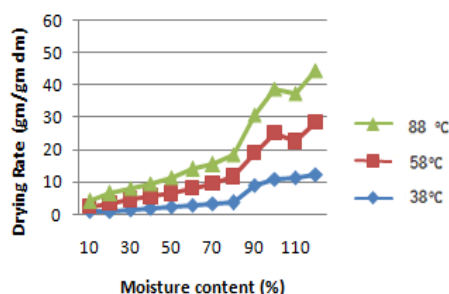
Fig. 2: Drying rate curve vs. moisture at the temperature range 38°C - 88°C, relative humidity of air 19.8-59.8% and air velocity of 1.1 m/sec., the effect of hotness on drying rate of bhindi and on drying time, if at higher value of moisture content, drying temperature increased then drying rate will increased and falling the drying time. The effect of relative humidity ratio of dryer, on drying time and drying rate, the drying rate of the bhindi increases with change of drying time, if humidity ratio were decreasing. This result with low humidity ratio of air for drying, diffusion of heat and mass in quantity wise required high and water loss is increases.
