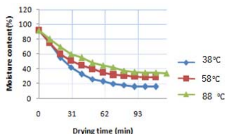
Fig. 1: Drying curve vs. time
