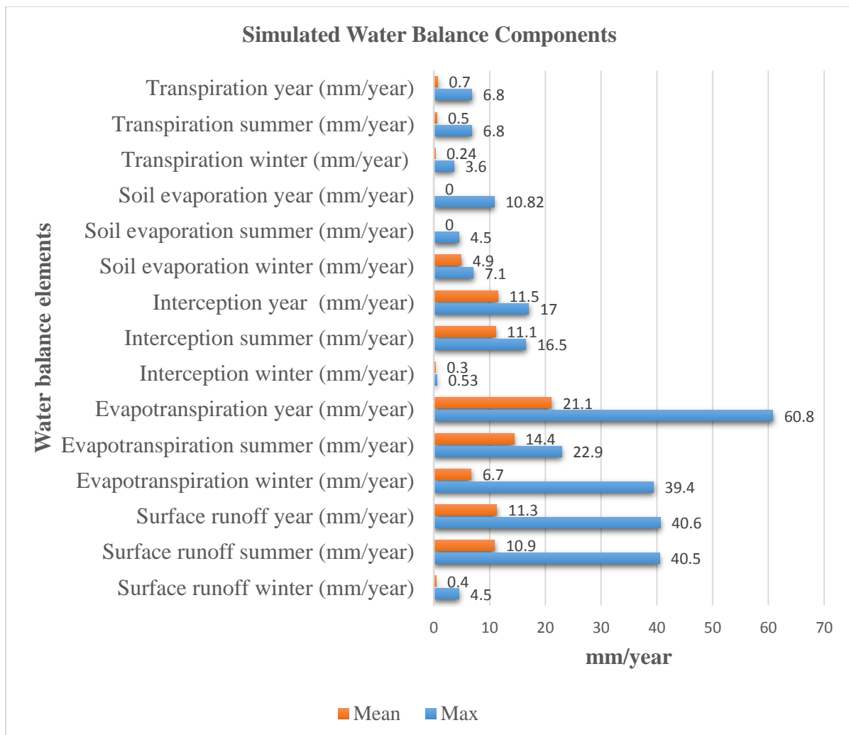
Figure 8: Water balance components simulated using WetSpass model for Birki watershed
