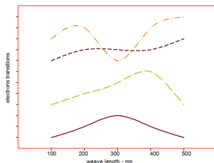
Fig. 1. Uv-Vis spectrum of complexes [\text{Mn}(\text{HQ})(\text{Dex})]\text{Cl}_2 , [\text{Mn}(\text{HQ})(\text{fru})]\text{Cl}_2 \pi \rightarrow \pi^* (brown dots), n \rightarrow \pi^* (brown line), d-d transition (light green dots) and C-T (orange dots)
