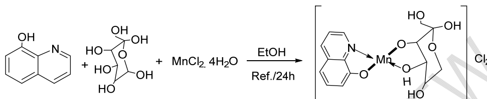
Scheme (2) preparation of [Mn(HQ)(Fru)]Cl_2
