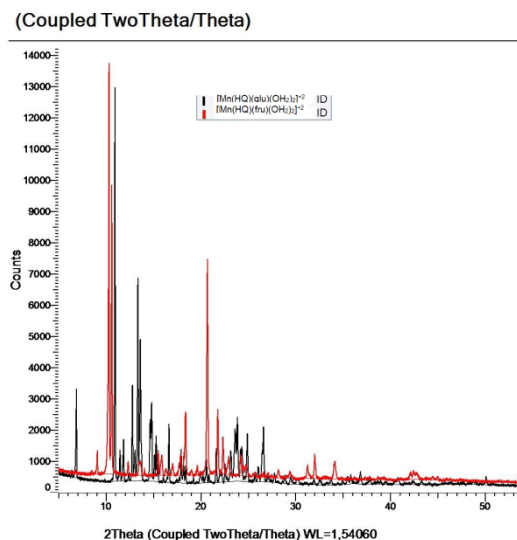
Fig. 2. XPRD spectra of [Mn(HQ)(Dex)]Cl_2 in Black and [Mn(HQ)(fru)]Cl_2 in red
