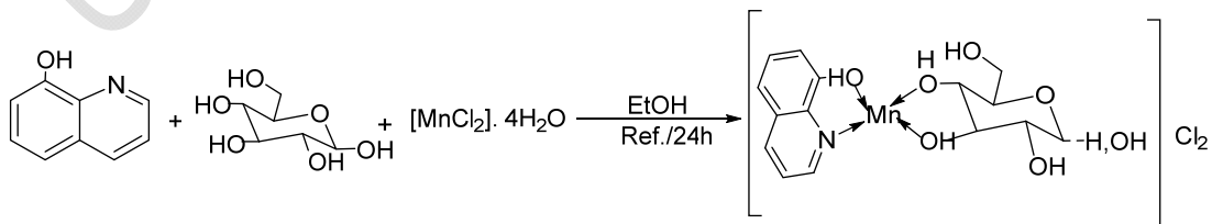
Scheme (1) preparation of [\text{Mn}(\text{HQ})(\text{Dex})]\text{Cl}_2
