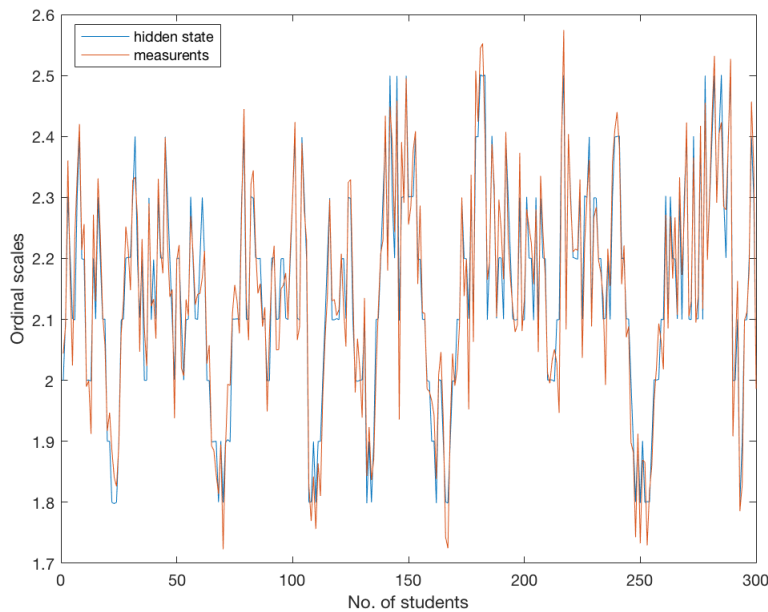
Figure 8: A plot of ordinal scale measurement and Hidden State
