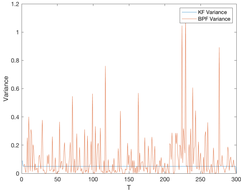
Figure 10: A plot of Kalman Filter and Monte Carlo variances
