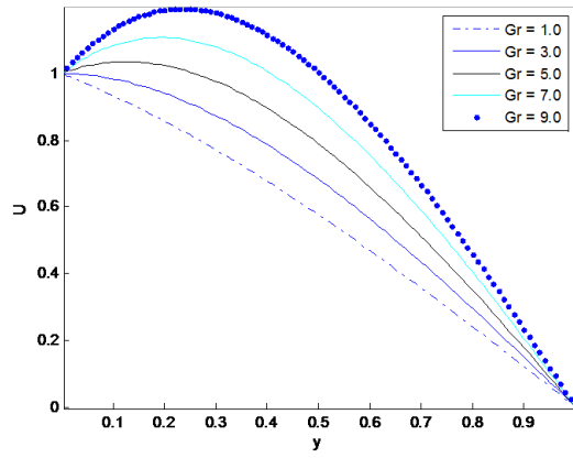
Figure 4: velocity profile for different values of Gr ( S = 2.0, \lambda = -0.2 )
