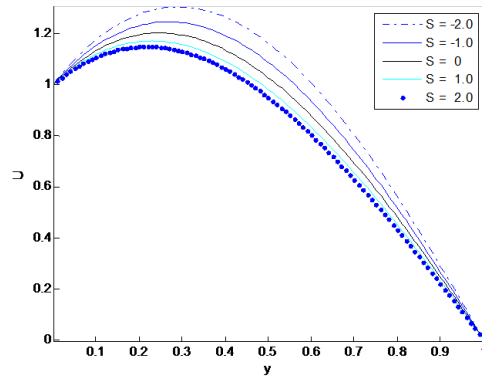
Figure 2: Velocity profile for different values of S ( Gr = 8.0, \lambda = -0.2 )
