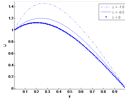
Figure 5: Velocity profile for different values of \lambda ( S = 2.0, Gr = 8.0 )
