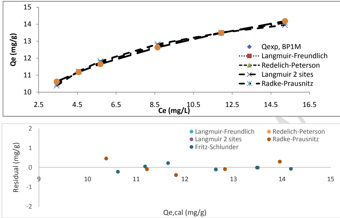
Figure 9: Non-linear isotherm and residual plot for more than two parameters in the case of BP1M.
