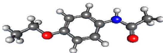
Figure 3: 3D structure of phenacetin.
