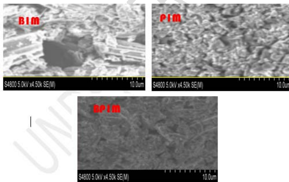
Figure 1: Electronic microscopy image of different activated carbon (BIM: activated carbon from ayous, PIM: activated carbon from egussi and BPIM: activated carbon from the mixture).
