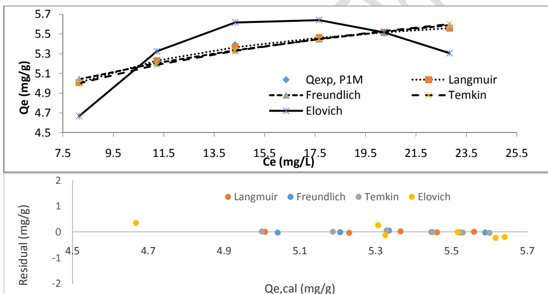
Figure 5: Non-linear isotherm and residual plot for two parameters in the case of P1M.
