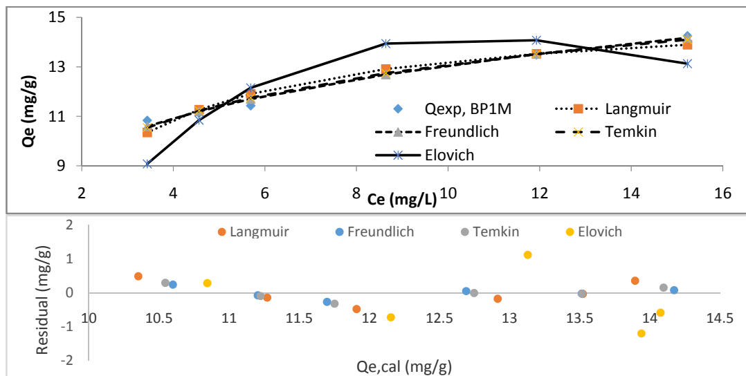
Figure 6: Non-linear isotherm and residual plot for two parameters in the case of BP1M.
