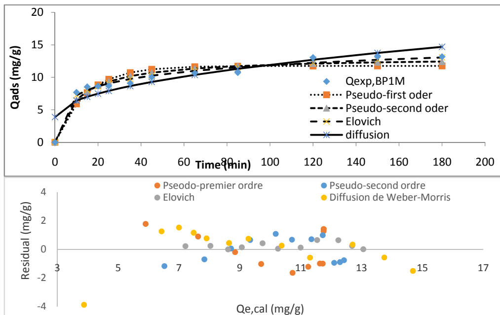
Figure 12: Non-linear kinetics models and residual plot in the case of BP1M.
