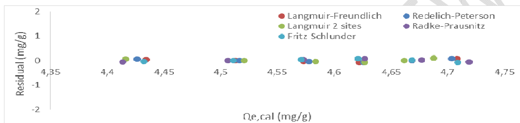
Figure 7: Non-linear isotherm and residual plot for more than two parameters in the case of B1M.
