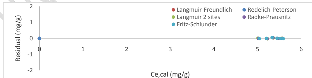
Figure 8: Non-linear isotherm and residual plot for more than two parameters in the case of P1M.
