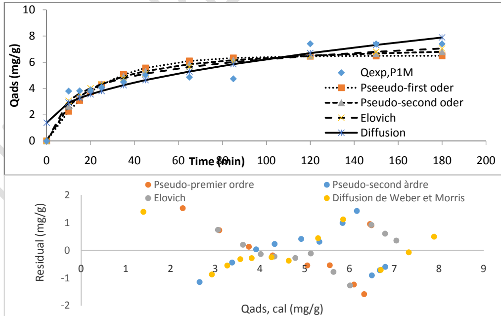
Figure 11: Non-linear kinetic models and residual plot in the case of P1M.
