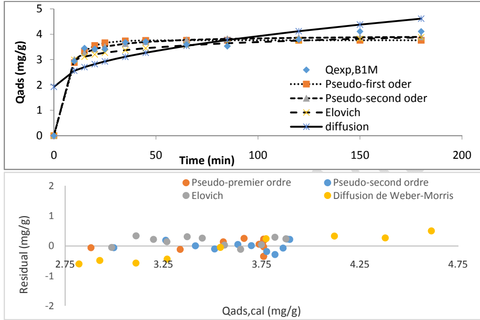
Figure 10: Non-linear kinetic models and residual plot in the case of B1M.
