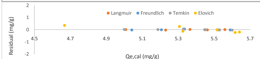
Figure 5: Non-linear isotherm and residual plot for two parameters in the case of P1M.
