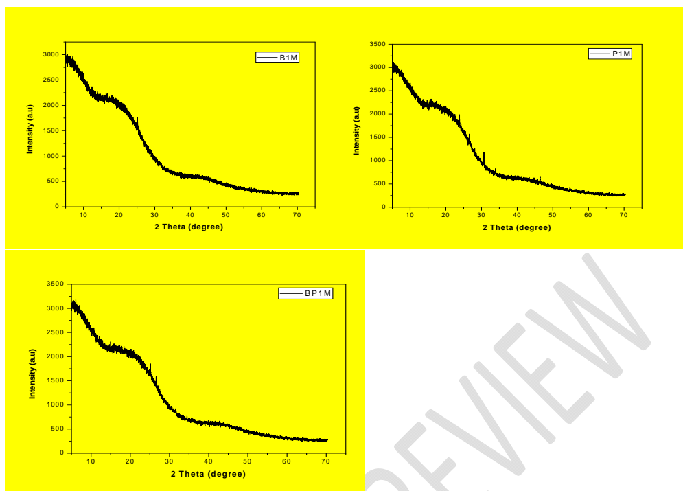
Figure 2: XRD spectrum of different activated carbon.
