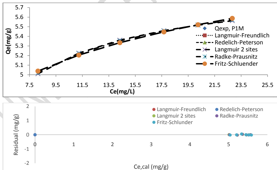
Figure 8: Non-linear isotherm and residual plot for more than two parameters in the case of P1M.
