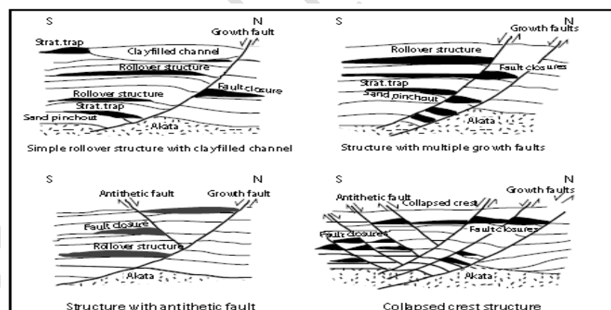
Fig. 4: Examples of Niger Delta oil field structures and associated trap types (Modified from [4] and [27].
