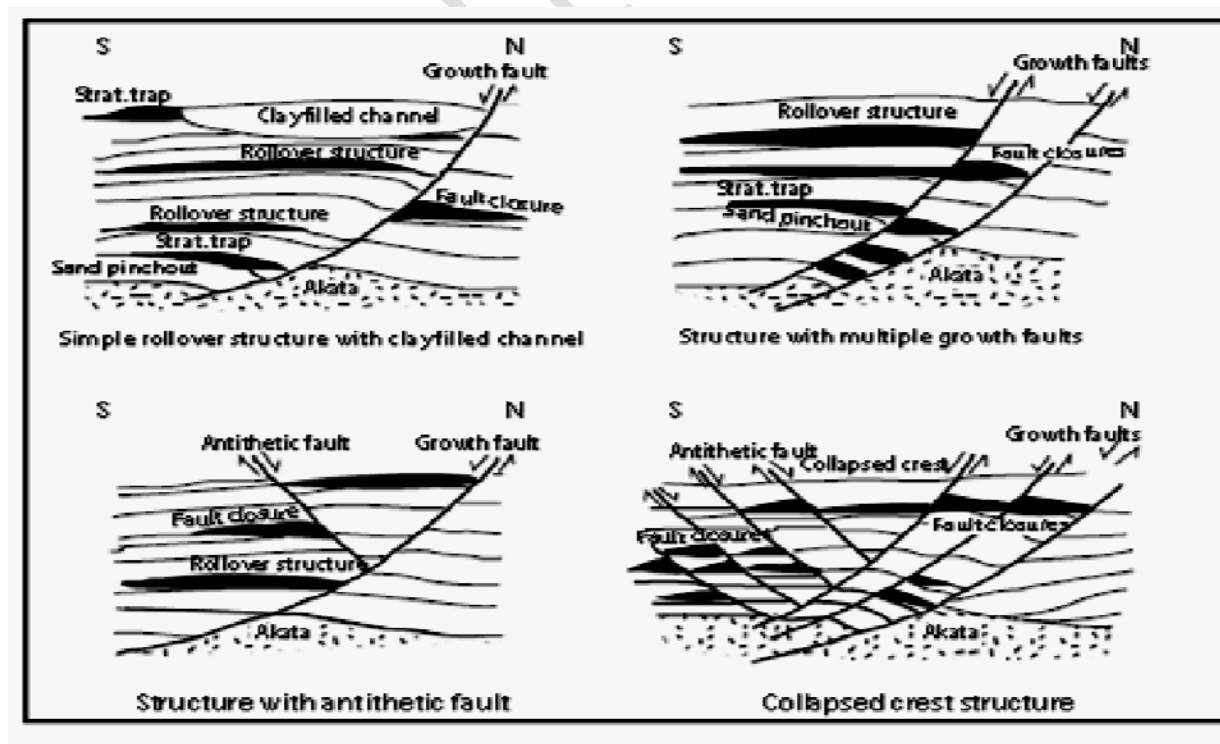
Fig. 4: Examples of Niger Delta oil field structures and associated trap types (Modified from [4] and [27].
