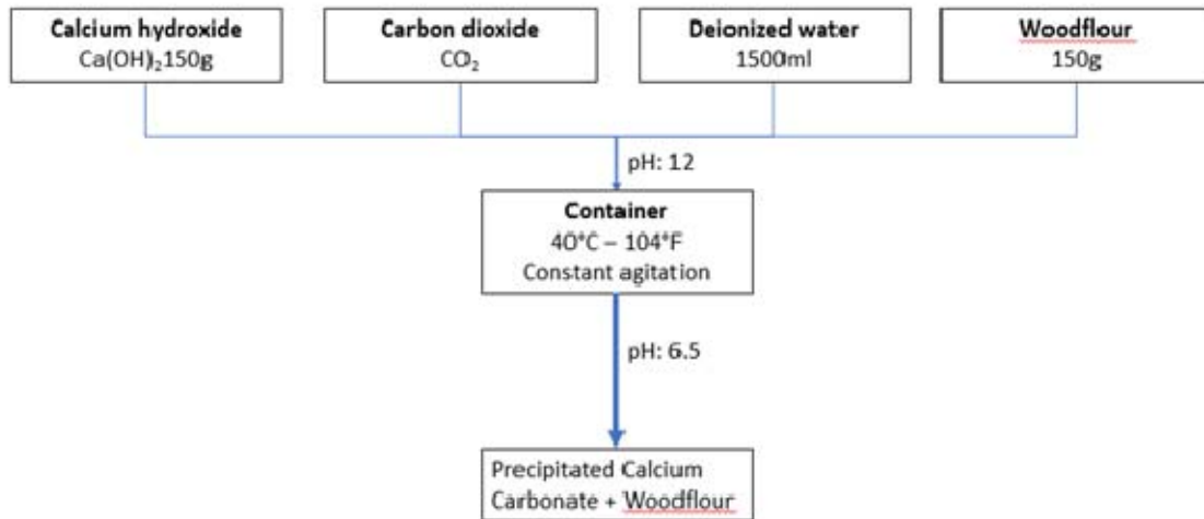
Fig. 1. PCC+ WF process sequence
