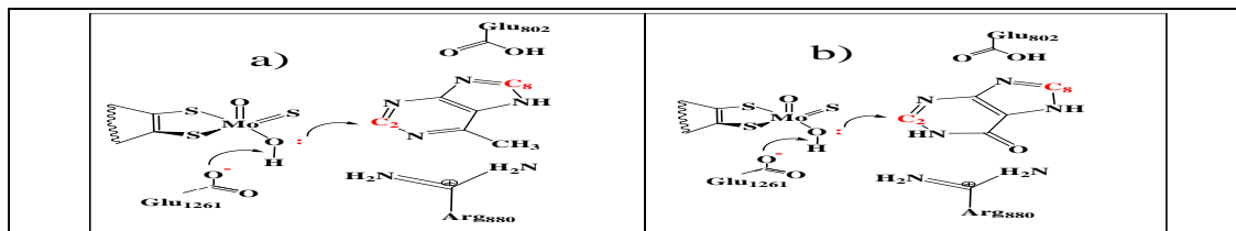
Figure 4.1.3. The orientation of 6-methylpurine and hypoxanthine inside the active site of xanthine oxidase enzyme.
