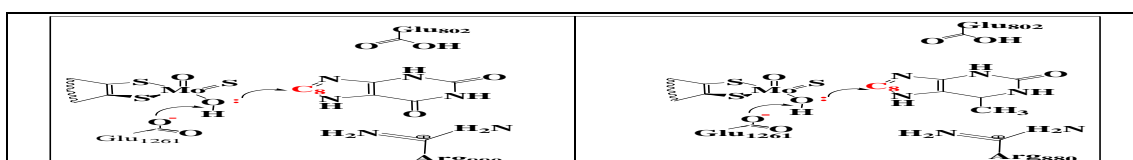
Figure 4.1.4. The orientation of xanthine and 2-hydroxy-6-methylpurine inside the active site of xanthine oxidase enzyme with the conserved binding pocket amino acid residues. Both xanthine and HMP bound to the Molybdenum center through the same interaction site at C 8 .
