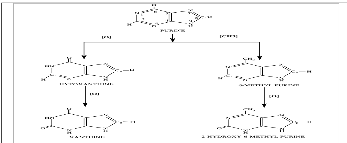
Figure 4.1.2. Purine and its derivatives. When purine oxidized and methylated at its C 6 position, it gives hypoxanthine and 6-methyl purine, respectively. Xanthine and HMP are the oxidized products of hypoxanthine and 6-methyl purine, respectively.
