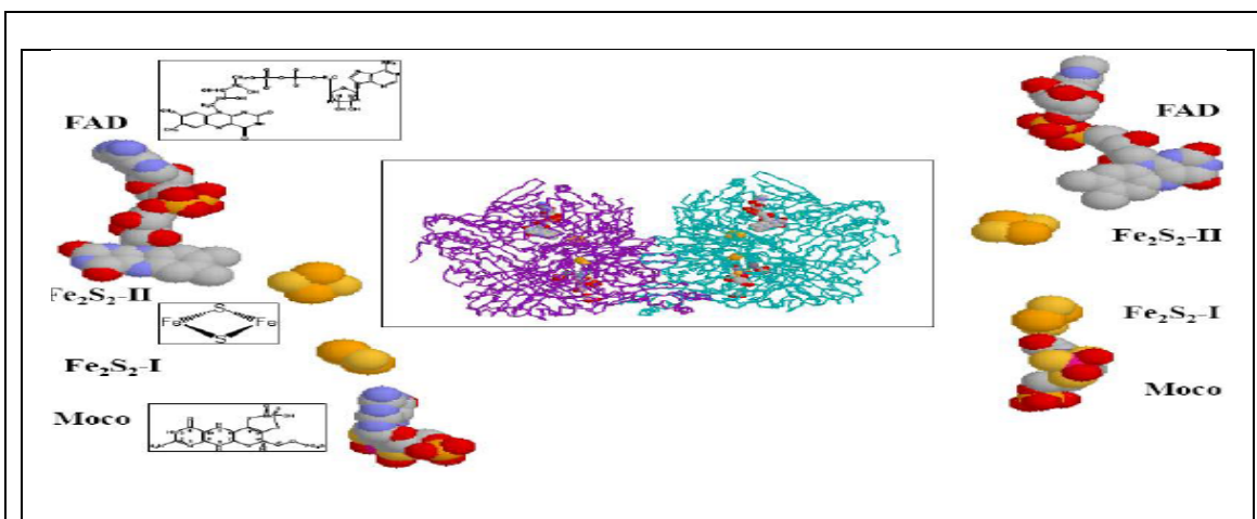
Figure 1. The overall structure ( center ) and cofactor compositions ( left and right ) of the bmXOR enzyme (PDB accession code of 1V97) [24] . Left and right display the linear arrangement of the cofactors: The FAD, pairs of [2Fe–2S], and Moco cofactors. The illustration is prepared with the application of protein explorer [13] .
