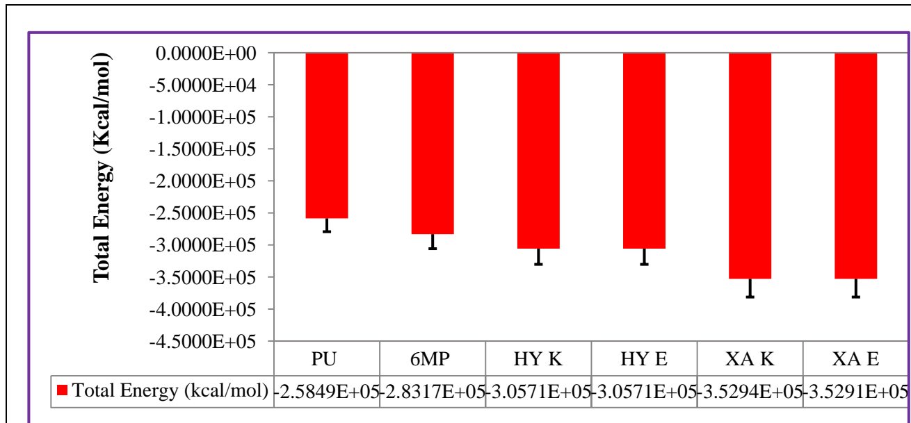
Figure 3.1.1. The total energy obtained from optimization purine derivatives (PU = Purine, HY E = Hypoxanthine enol, HY= Hypoxanthine keto, 6MP = 6-Methylpurine, XA E = Xanthine enol, and XA K = Xanthine keto). The plot was generated from the raw data shown in Appendix (A, Table A.II.2).
