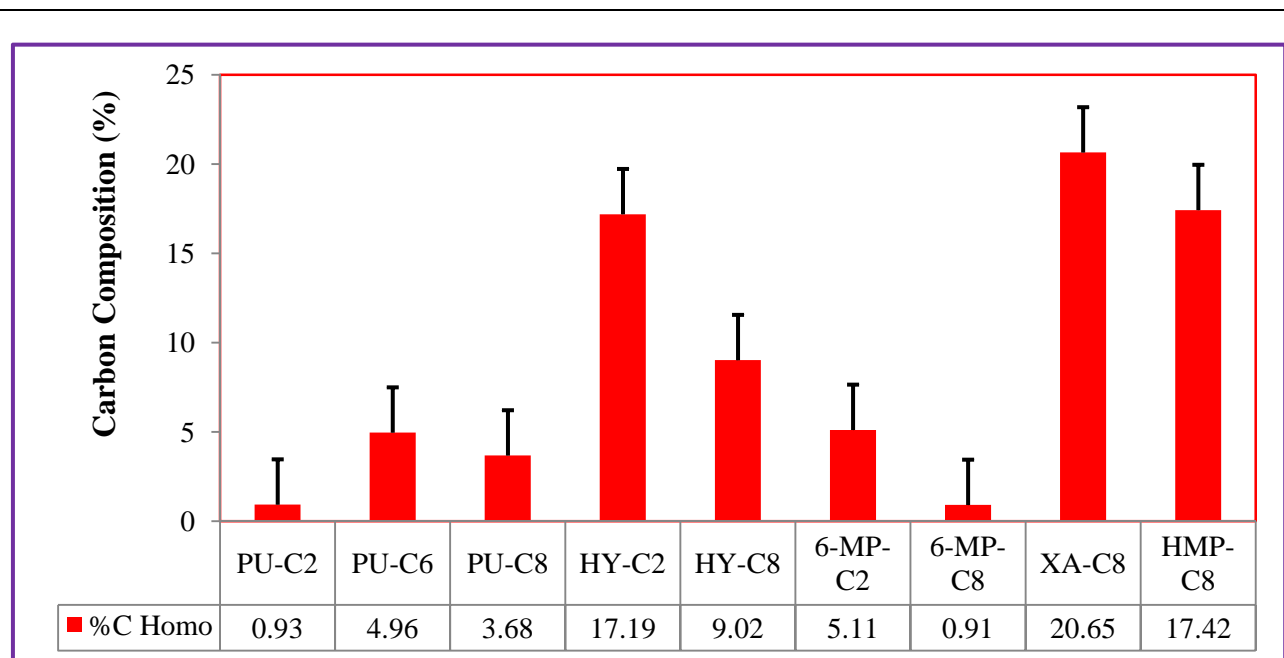
Figure 3.1.9. The percent compositions of carbon, on HOMO, determined on the interaction sites (at C 2 and C 8 ). The data were obtained from AOMix software package.
