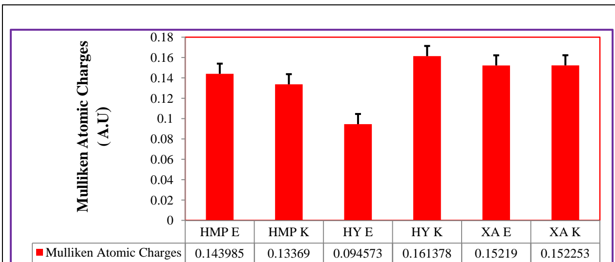
Figure 3.1.3. The Mulliken atomic charges probed at the most favorable interaction sites of purine derivatives. The plot was developed from the raw data shown in Appendix (A, Table A.II.1).
