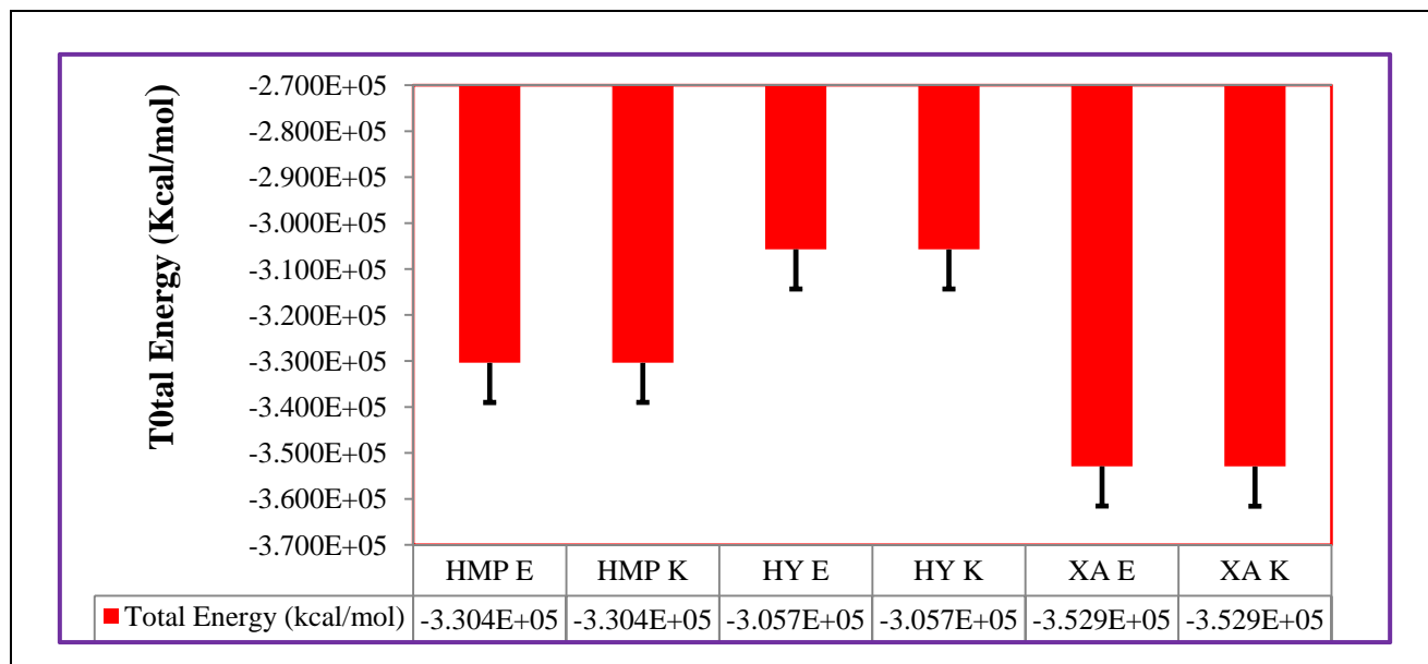
Figure 3.1.2. The total energy obtained from optimization of the oxidized forms of purine derivatives (HMP E, HMP K, HY E, HY K, XA E and XA K).
