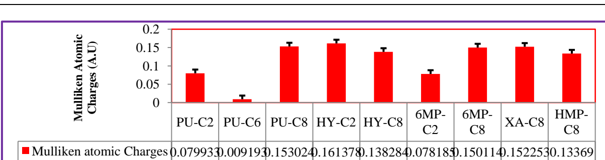
Figure 3.1.7. Comparison of Mulliken atomic charges, on the interaction sites at C 2 and C 8 , for purine derivatives (purine, hypoxanthine, 6-methylpurine, xanthine and 2-hydroxy-6-methylpurine, respectively). The plot was developed from the raw data shown in Appendix (A, Table A.II.1).
