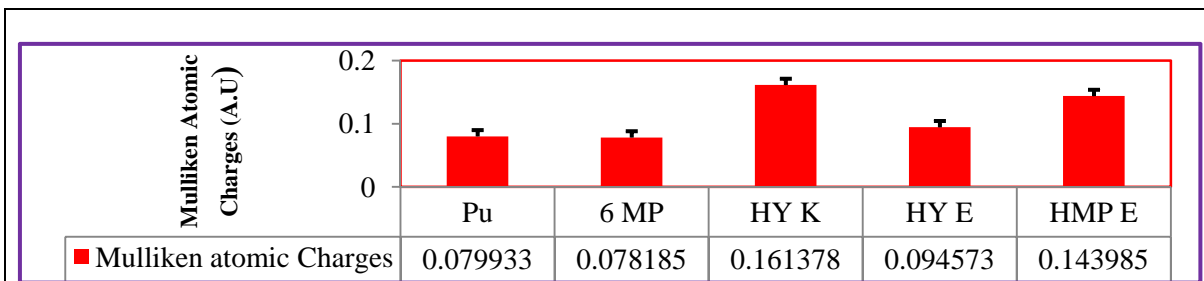
Figure 3.1.5. Comparison of Mulliken atomic charges, on the interaction sites at C 2 , for the keto and enol tautomers of purine and its derivatives (MP, HMP, and HY). The plot was developed from the raw data shown in Appendix (A, Table A.II.1).
