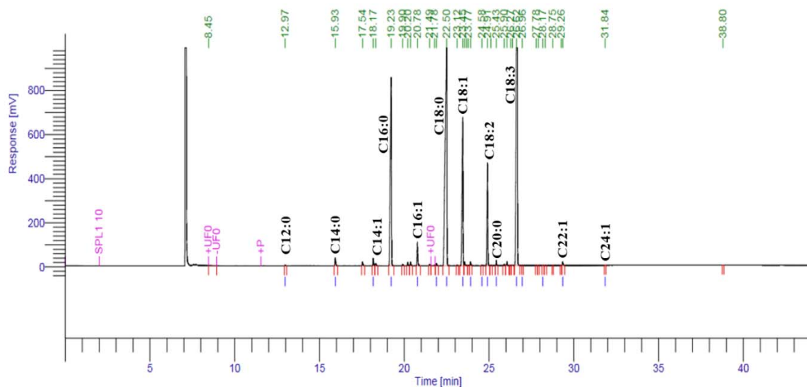
Fig. 2. Gas chromatograms of fatty acids methyl esters of C. butyrospermi oil analysed
