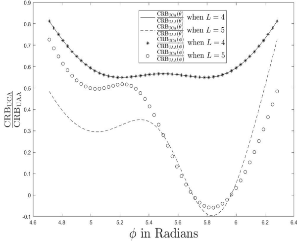
Fig. 6. \frac{\text{CRB}_{\text{UCA}}(\theta)}{\text{CRB}_{\text{UAA}}(\theta)} < 1 and \frac{\text{CRB}_{\text{UCA}}(\phi)}{\text{CRB}_{\text{UAA}}(\phi)} < 1 when L = 4 and 5 and \frac{3}{2}\pi \leq \phi \leq 2\pi
