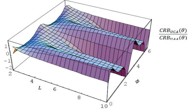
Fig. 3. Comparison of \text{CRB}_{\text{UCA}}(\theta) and \text{CRB}_{\text{UAA}}(\theta) .
