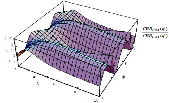
Fig. 4. Comparison of \text{CRB}_{\text{UCA}}(\phi) and \text{CRB}_{\text{UAA}}(\phi) .
