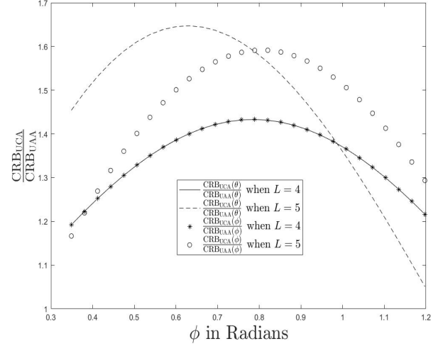
Fig. 7. \frac{\text{CRB}_{\text{UCA}}(\theta)}{\text{CRB}_{\text{UAA}}(\theta)} > 1 and \frac{\text{CRB}_{\text{UCA}}(\phi)}{\text{CRB}_{\text{UAA}}(\phi)} > 1 when L = 4 and 5 and \frac{\pi}{9} \leq \phi \leq \frac{7}{18}\pi
