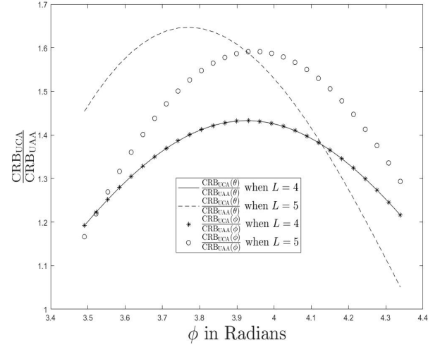
Fig. 8. \frac{\text{CRB}_{\text{UCA}}(\theta)}{\text{CRB}_{\text{UAA}}(\theta)} > 1 and \frac{\text{CRB}_{\text{UCA}}(\phi)}{\text{CRB}_{\text{UAA}}(\phi)} > 1 when L = 4 and 5 and \frac{10}{9}\pi \leq \phi \leq \frac{25}{18}\pi
