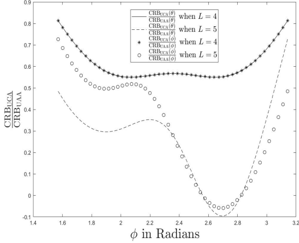
Fig. 5. \frac{\text{CRB}_{\text{UCA}}(\theta)}{\text{CRB}_{\text{UAA}}(\theta)} < 1 and \frac{\text{CRB}_{\text{UCA}}(\phi)}{\text{CRB}_{\text{UAA}}(\phi)} < 1 when L = 4 and 5 and \frac{\pi}{2} \leq \phi \leq \pi
