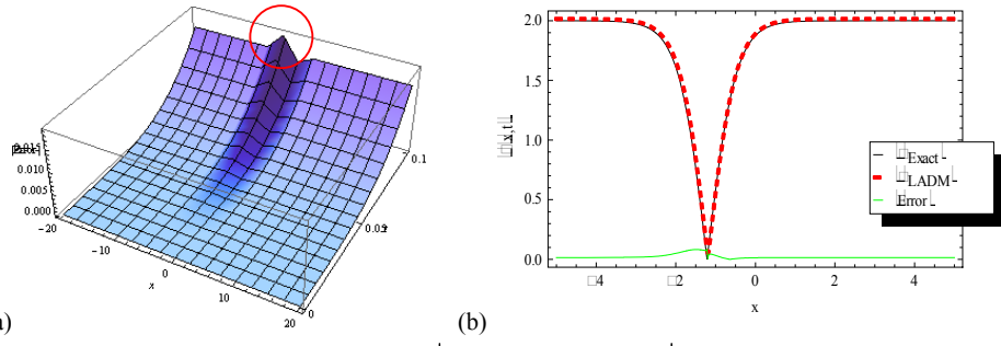
Figure 2. The plots of : (a) The error module |\Psi(x,t) - \Psi_{LDM}(x,t)| . (b) The peak of the Error Module Curve when t = 0.1 .
