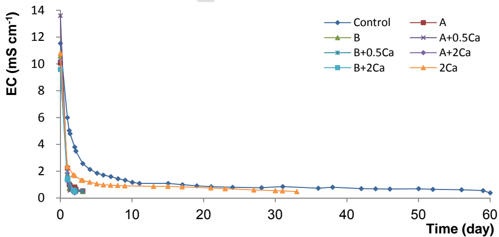
Fig. 3. Periodical change of electrical conductivity (EC) in the eluents from soil columns
