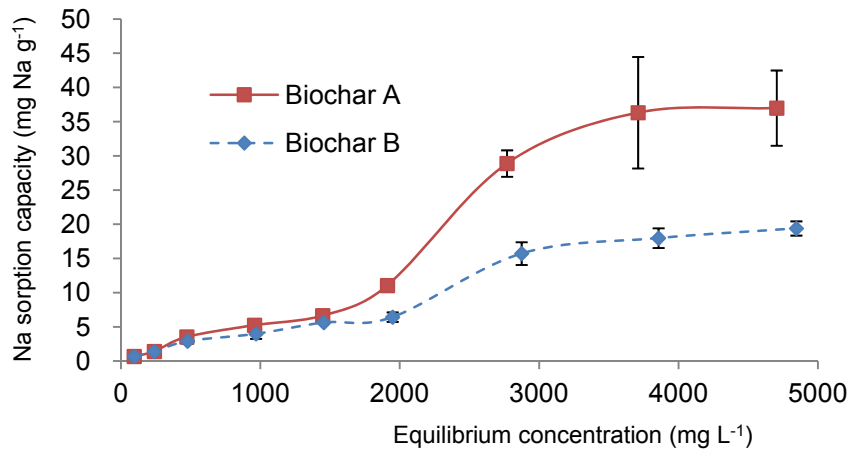
Fig. 8. Sorption isotherm of Na + on two different biochars ( P < .001 ). Bars represent standard deviation of n = 4 .
