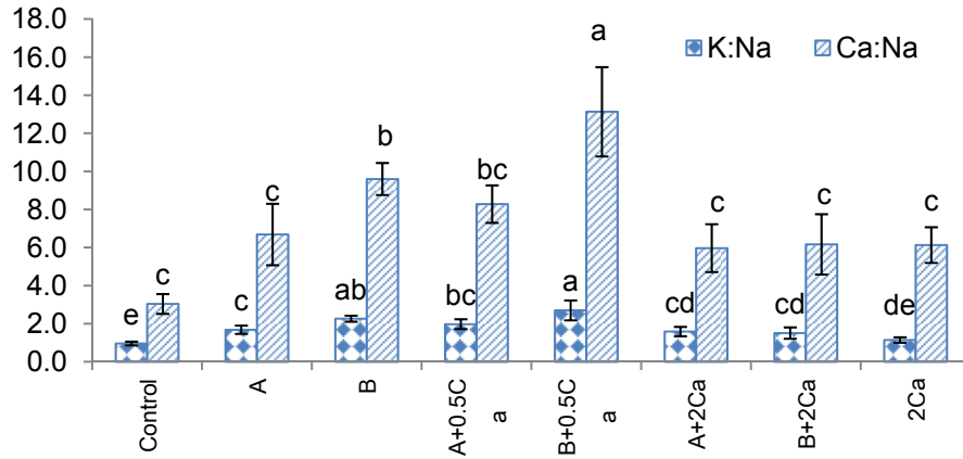
Fig. 7. Change in K:Na and Ca:Na ratios of soil after leaching
