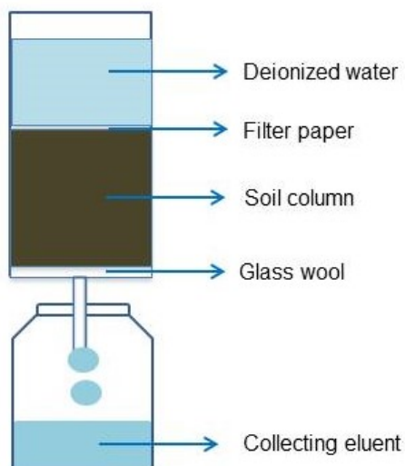
Fig. 1. Experimental apparatus
