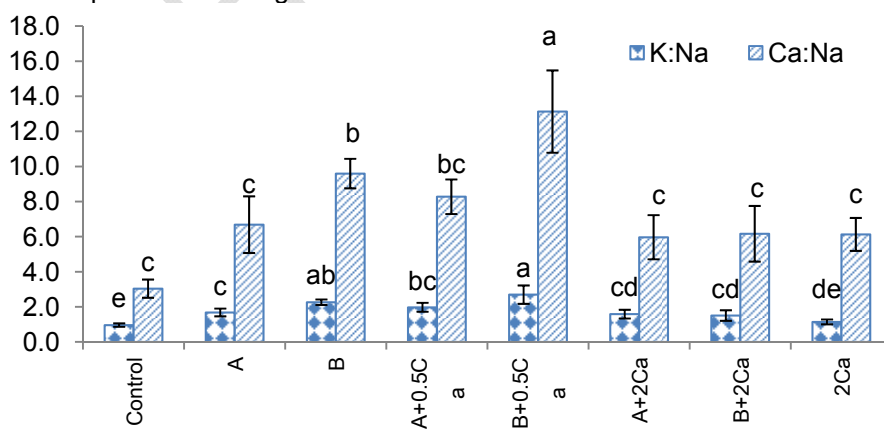
Fig. 7. Change in K:Na and Ca:Na ratios of soil after leaching
