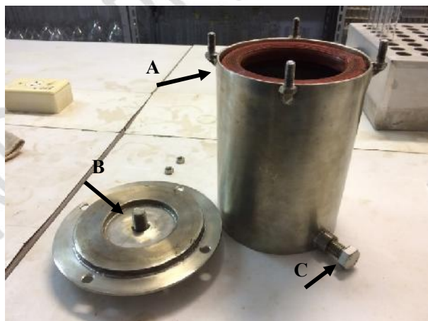
Fig. 1. Inox chamber used for pyrolysis in the non-oxidizing condition. A: Cap seal; B: N2 input; C: Chamber air outlet, Cuiabá, Mato Grosso, Brazil
