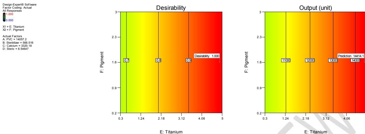
Figure 8: Desirability User defined Solution Minimum run Characterization design in Factorial design method shows the approximation of the desirability on the optimal solution in the production system. Minimum run Characterization design in Factorial design method shows the approximation of the output on the optimal solution in the production system.
