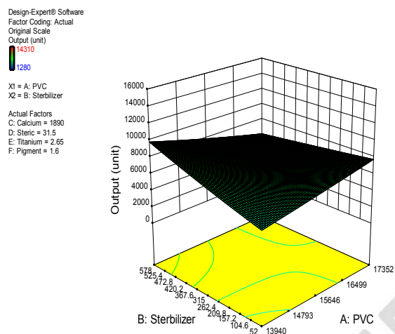
Figure 3a: The 3D Surface Plot for PVC and Stabilizer
