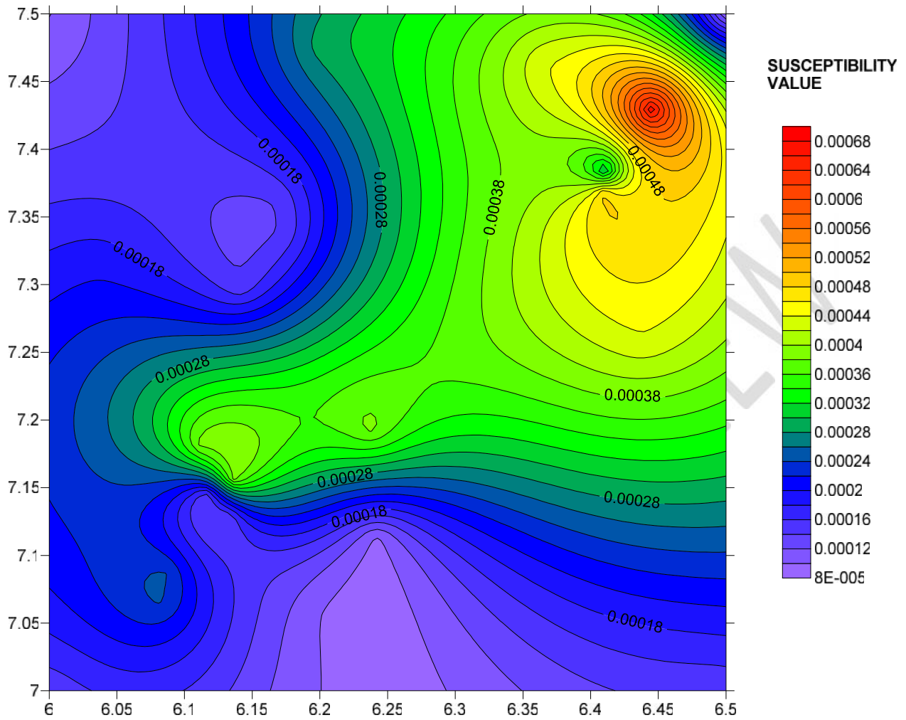
Fig.5. Magnetic Susceptibility map of the Study Area Showing Rock Contrasts
