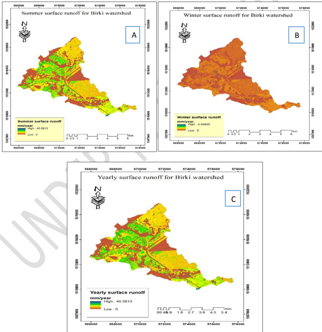
Figure 5: Summer (A), winter (B) and annual (C), surface runoff simulated for Birki watershed
