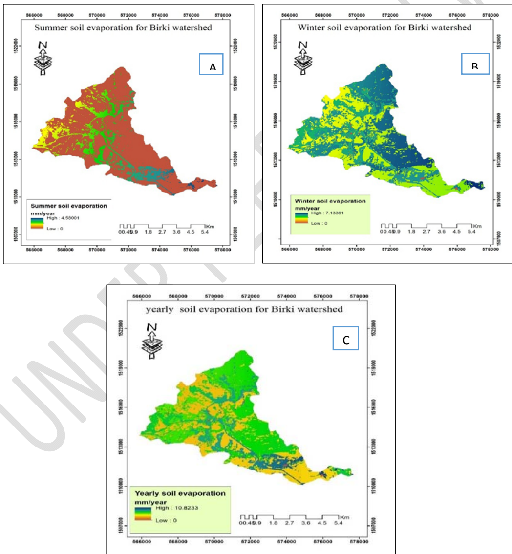
Figure 7: Summer (A), winter (B) and annual (C), Soil evaporation simulated for Birki watershed.
