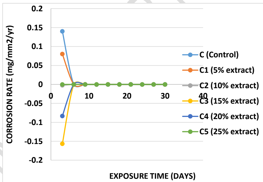
Figure 2: Plot of corrosion rate for gray cast iron samples immersed in 0.5M NaOH with or without water hyacinth extract as inhibitor
