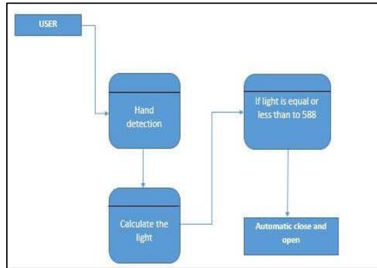
Figure 9: SMARTBin Data Flow Diagram
