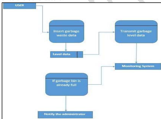
Figure 8: SMS Notification Data Flow Diagram
