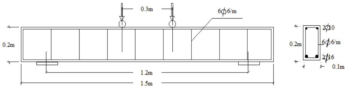
Fig. 4: Testing setup for beams
