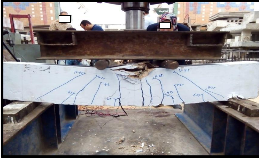
Fig.7: Sample of cracks propagation and mode of failure.
