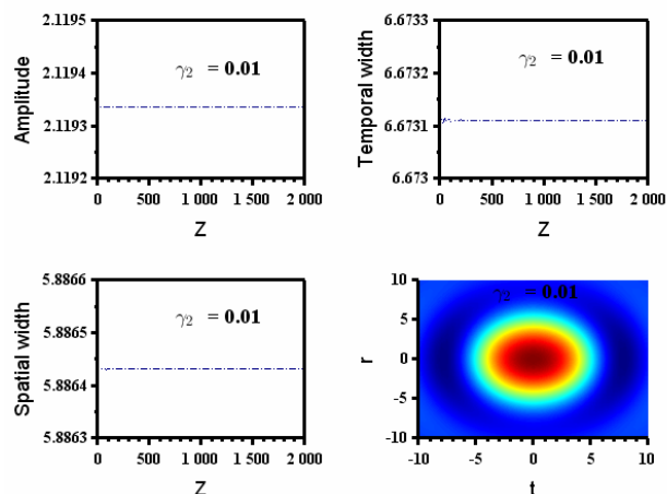
Figure 7. Evolution of stationary soliton amplitude, spatial and temporal widths for the higher-order spectral filter \gamma_2 = 0.01 . The values of other parameters are D = \gamma = 1 , \beta = -0.3 , \delta = -0.5 , \mu = -0.1 , \nu = -0.252 and \varepsilon = 0.508 .
