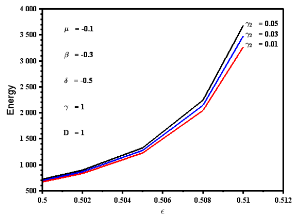
Figure 3. Evolution of the total energies of stationary dissipative solitons for different values of the higher-order spectral filter term. The red curve corresponds to \gamma_2 = 0.01 , blue to \gamma_2 = 0.03 , and black to \gamma_2 = 0.05 . The values of other parameters are D = \gamma = 1 , \beta = -0.3 , \delta = -0.5 , \mu = -0.1 and v = -0.252 .
