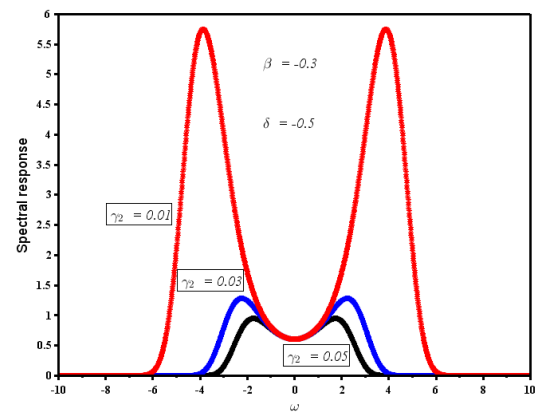
Figure 1. Spectral responses evolution according to the values of the higher-order spectral filter term \gamma_2 . Red: \gamma_2 = 0.01 , blue: \gamma_2 = 0.03 , and black: \gamma_2 = 0.05
