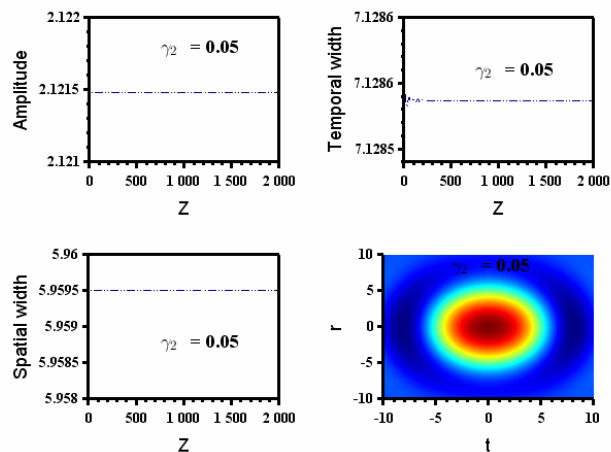
Figure 5. Evolution of stationary soliton amplitude, spatial and temporal widths for the higher-order spectral filter \gamma_2 = 0.05 . The values of other parameters are D = \gamma = 1 , \beta = -0.3 , \delta = -0.5 , \mu = -0.1 , \nu = -0.252 and \varepsilon = 0.508 .
