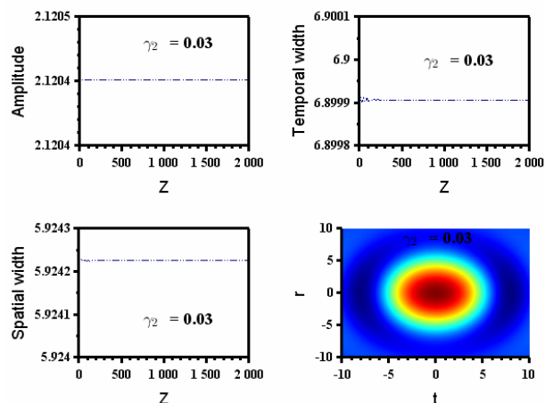
Figure 6. Evolution of stationary soliton amplitude, spatial and temporal widths for the higher-order spectral filter \gamma_2 = 0.03 . The values of other parameters are D = \gamma = 1 , \beta = -0.3 , \delta = -0.5 , \mu = -0.1 , \nu = -0.252 and \varepsilon = 0.508 .
