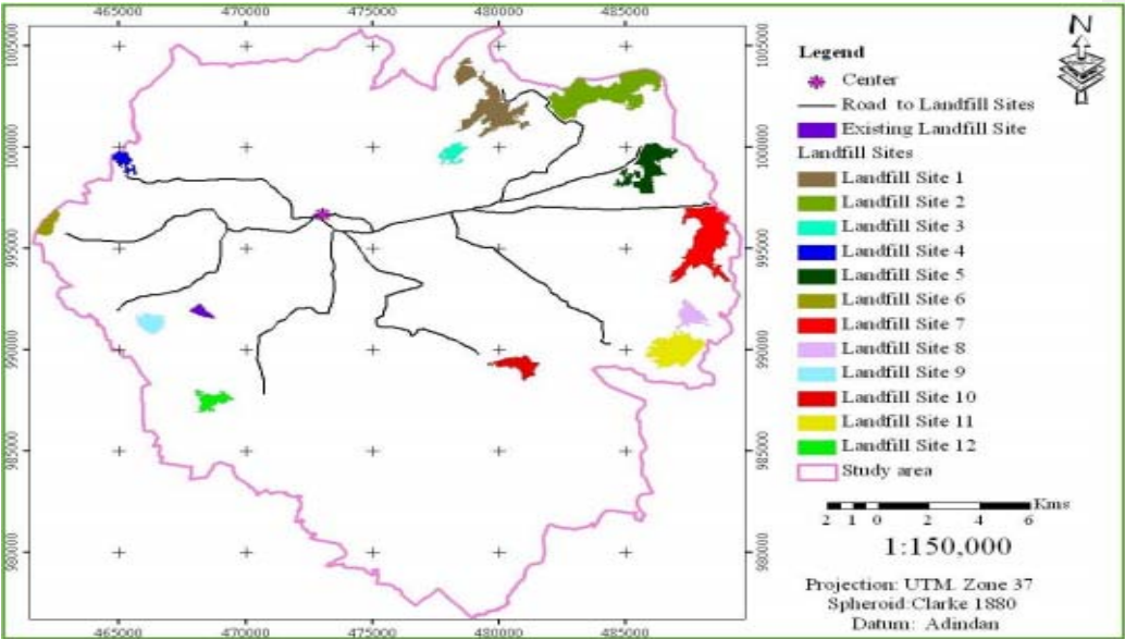
454 455 Figure 12: Final sustainability solid waste dumping landfill site selection by using GIS
