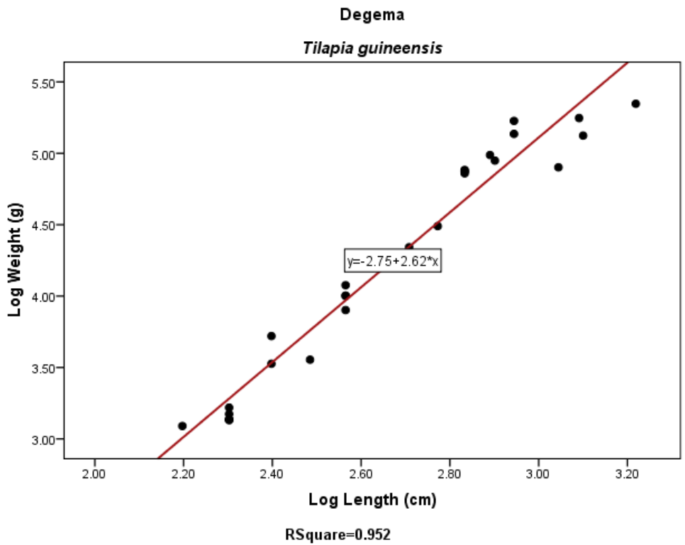
Fig 8: Log Length and Log Weight relationship (Bivariate Fit) of Tilapia guineensis in Degema
