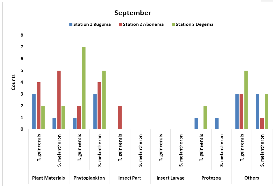
Fig 2: Stomach Content Analysis for September 2018.
