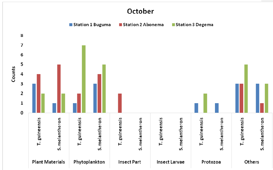
Fig 3: Stomach Content Analysis for October 2018.
