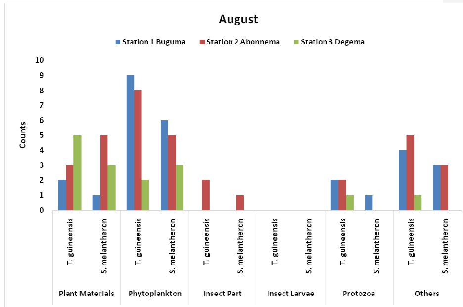
Fig 1: Stomach Content Analysis for August 2018.
