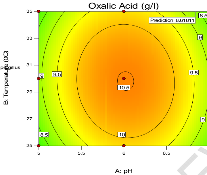
Fig. 1: Optimal response surface plot of oxalic acid production as a function of pH, temperature and substrate
