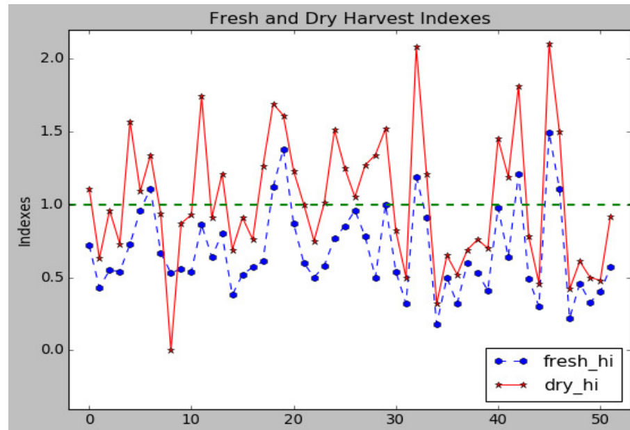
Figure 13: Harvest index comparison.
