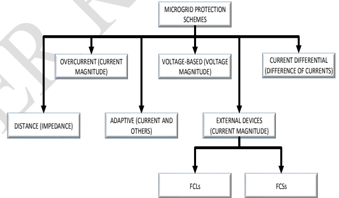
Fig. 1. Classification of protective schemes for microgrids.
