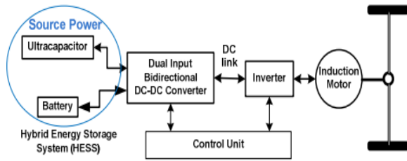
Figure 3 Block diagram of power circuit of EV with HESS
