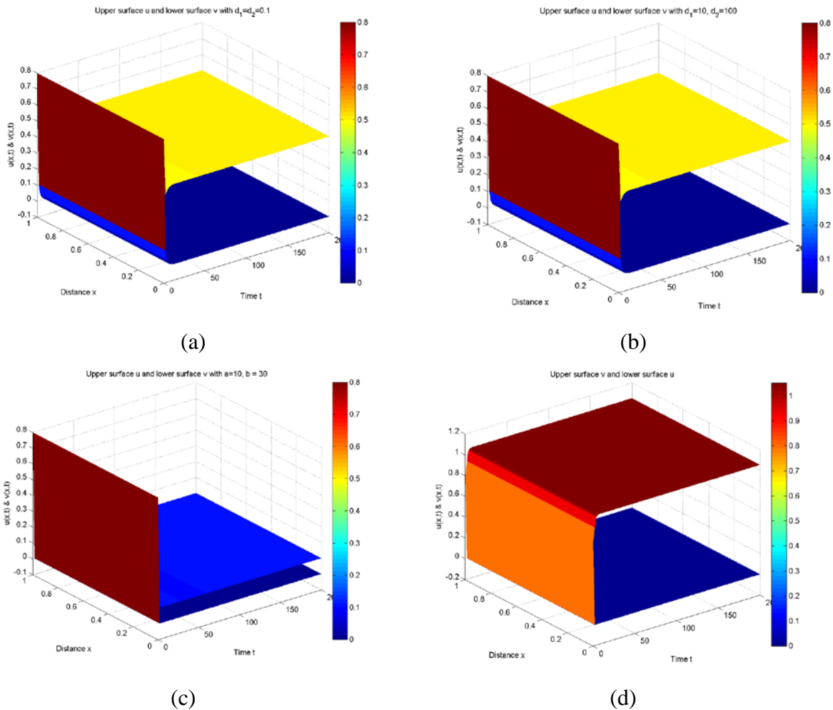
Figure 3.1: Dynamics of the system of equation (3.1) which corresponds (1.1) for various changes of parameter.
