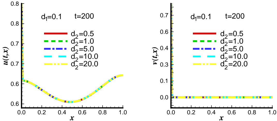
Figure 3.6: Solutions of (3.2) for d_1=0.1 , \sigma = (0,1) , u_0 = v_0 = 0.8 for various d_2=0.5, 1.0, 5.0, 10.0 and 20.0 at time t = 200 .
