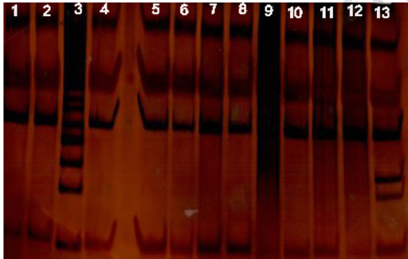
Fig. 1: Sequence polymorphism analysis of a PCR-restricted fragment of the FOLH1 gene in rs61886494 locus after enzymatic digestion using a MseI restriction enzyme, well 3: 50 bp DNA marker, (Sinaclon Co.), well 13: the heterozygote CT and the rest of the wells (wells 1-12) associated with homozygous CC in schizophrenic patients
