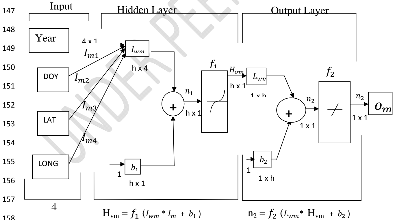
Figure 2: Schematic Diagram of Neural Network Training Window
