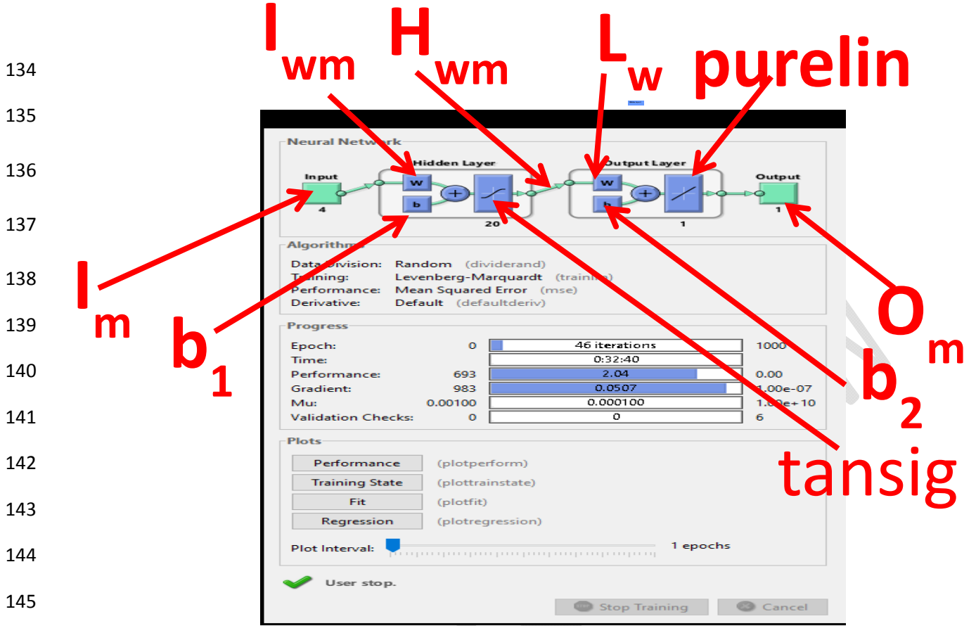
Figure 2: Schematic Diagram of Neural Network Training Window
