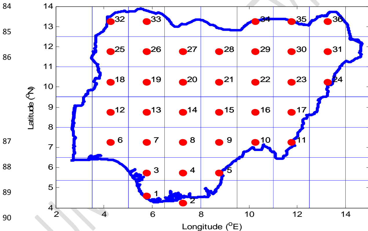
91 Figure 1: Gridded Map Showing Data Points of the selected stations in Nigeria
