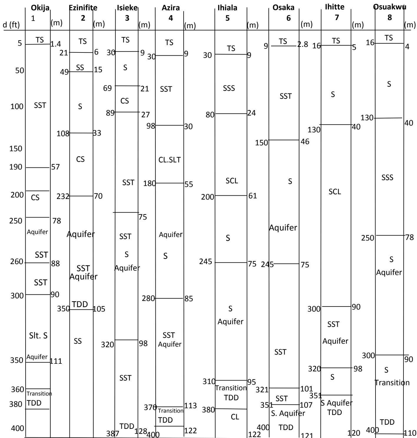
Fig 2. Aquifer Litho-logical Units of Different Locations in the Area
