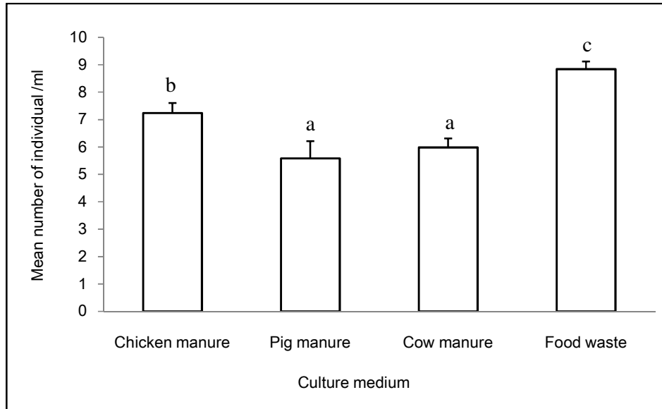
Fig. 2. Mean population growth of M. macrocopa cultured in 1000ppm concentration of four culture medium. Values are the ( mean \pm SD ). Different subscripts denote significant differences at P < 0.05 (a < b < c) .
