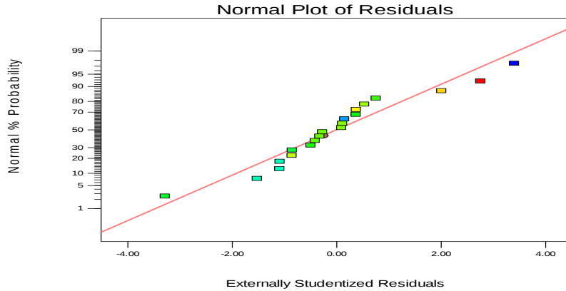
Figure 3: Normal plot of Residuals of the optimization process
