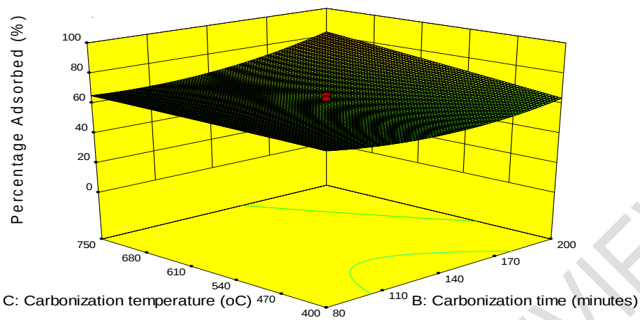
Figure 4: Interactive effects of temperature and time
