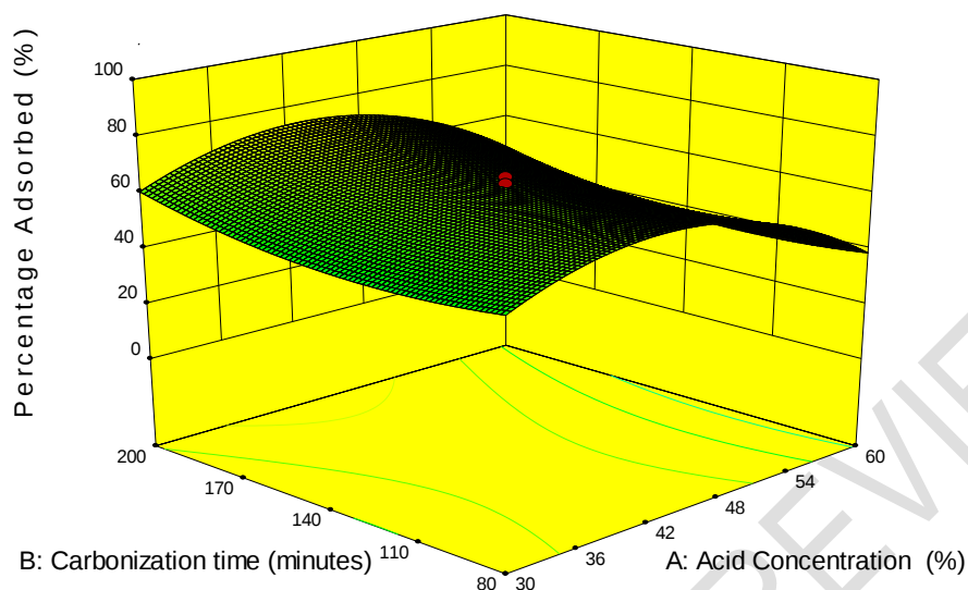
Figure 6: Interactive effects of time and concentration
