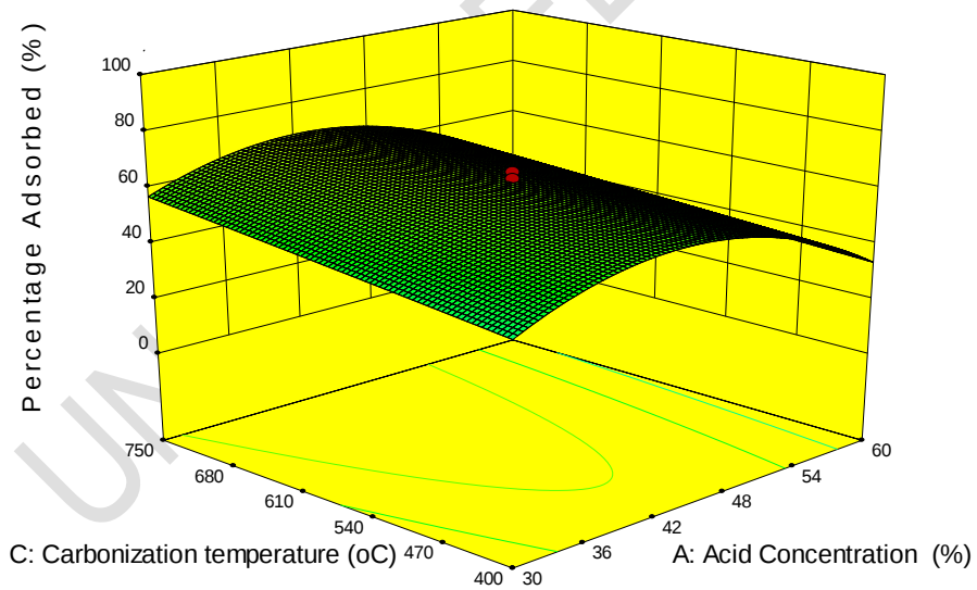
Figure 5: Interactive effect of temperature and concentration
