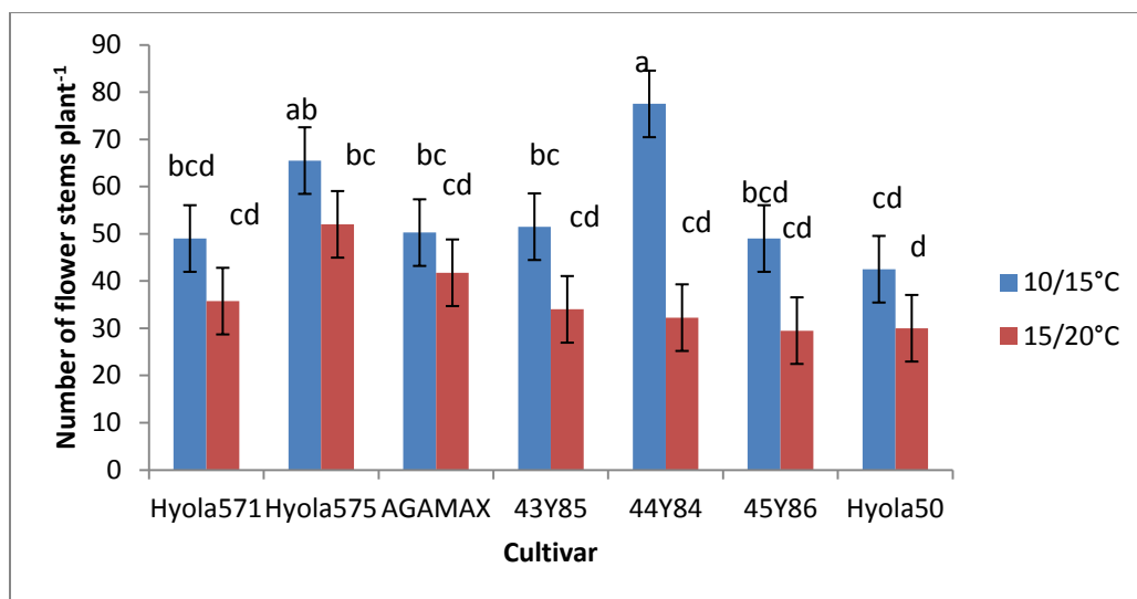
Figure 5 Flower stems plant -1 of different canola genotypes, measured during the final harvest at growth stage 5.4 in response to night/ day temperatures of 10/15°C and 15/20°C. Values with the same alphabetical lettering do not differ significantly at P=0.05
