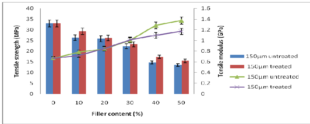
Figure 1: Effect of filler loading on the tensile strength and modulus of NaOH treated and untreated date pits/ epoxy composites.
