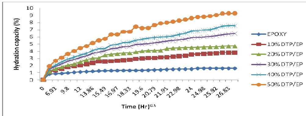
Figure 4: Water absorption curves of untreated date pits/ epoxy composite.
