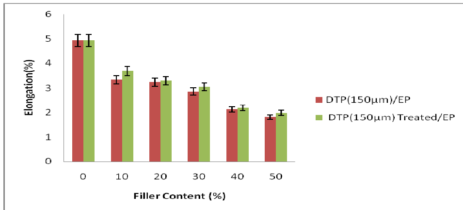
Figure 2: Effect of filler loading on the percentage elongation at break of NaOH untreated and treated date pit/ epoxy (DTP/ EP) composites.
