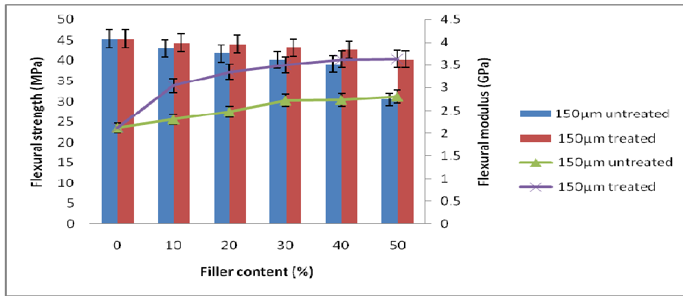
Figure 3: Effect of filler loading and particle size on the flexural strength and modulus of treated and untreated date pits/ epoxy composites.
