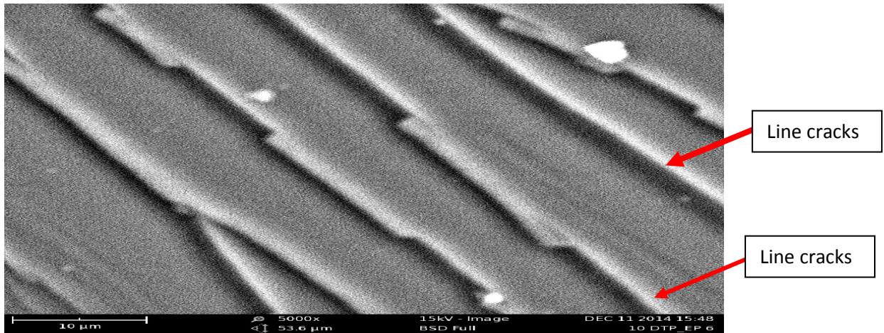
Plate 5: SEM micrograph of the fracture surface of 10 % treated date pits filler /epoxy composite at 5000x Magnification
