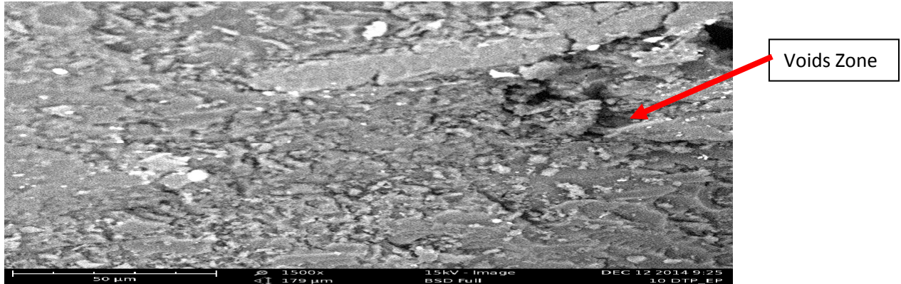
Plate 2: SEM micrograph of the fracture surface of 10% date pits filler /epoxy composite at 1500x Magnification.
