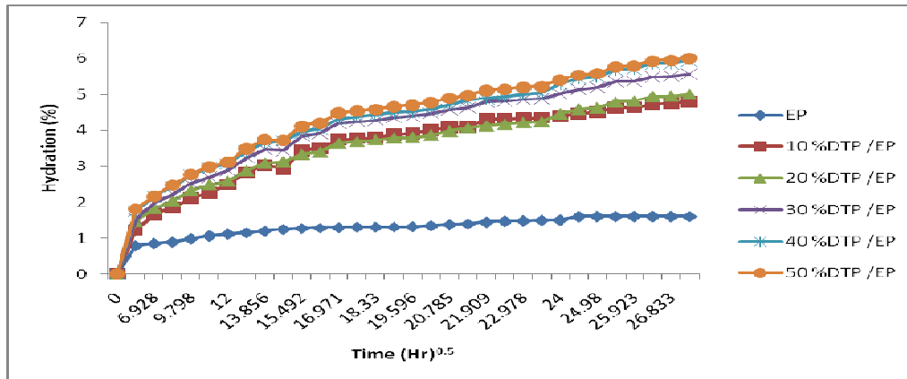
Figure 4: Water absorption curves of untreated date pits/ epoxy composite.
