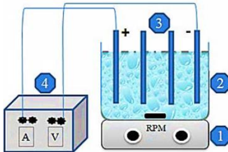
Fig 2: Bench-scale EC reactor with bipolar electrodes in parallel connection 1. Magnetic stirrer 2. EC reactor 3. Bipolar electrodes 4. DC power supply
