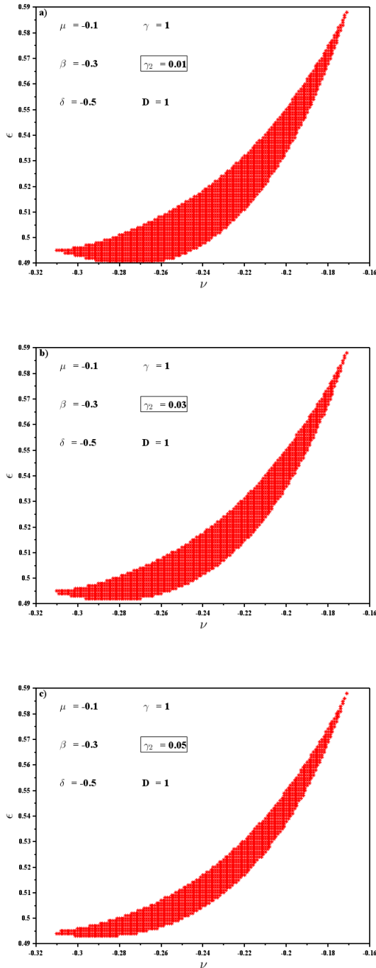
Figure 2. Cartographies of the solutions of the 2D complex Swift-Hohenberg equation in the (v, \varepsilon) plane. The stable fixed points regions in red represent the domain of stationary solitons. Other CSHE parameters appear inside the Figure 2.
