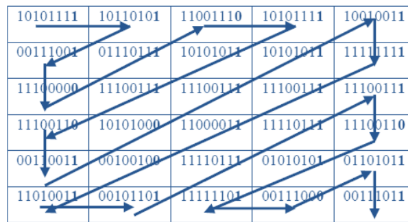
Fig 2: Basic Zigzag Scanning Process
