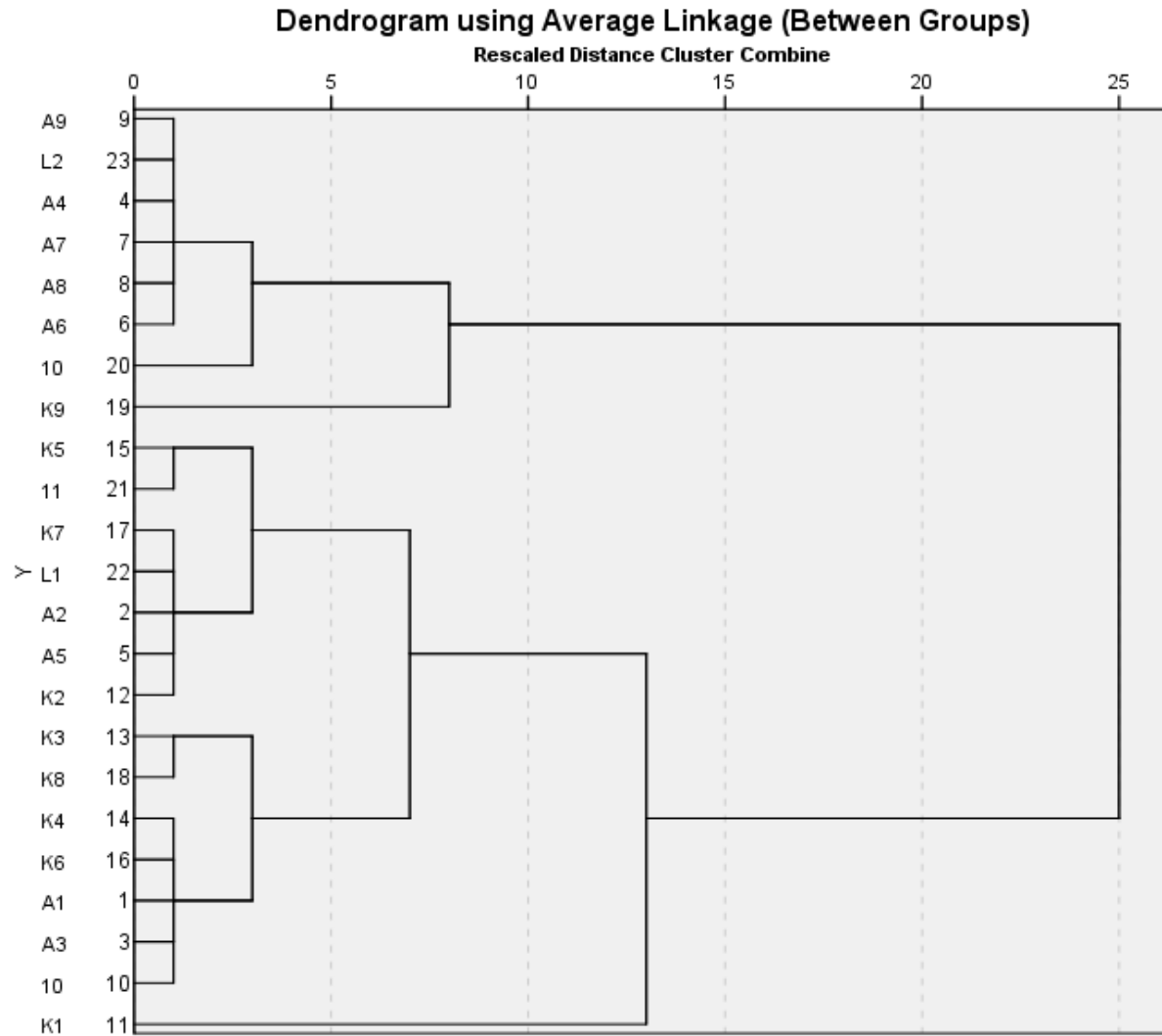
Figure 2: Dendrogram of 16srRNA of Extended Spectrum Beta-lactamase producing Escherichia coli after digestion with endonuclease BspI .
