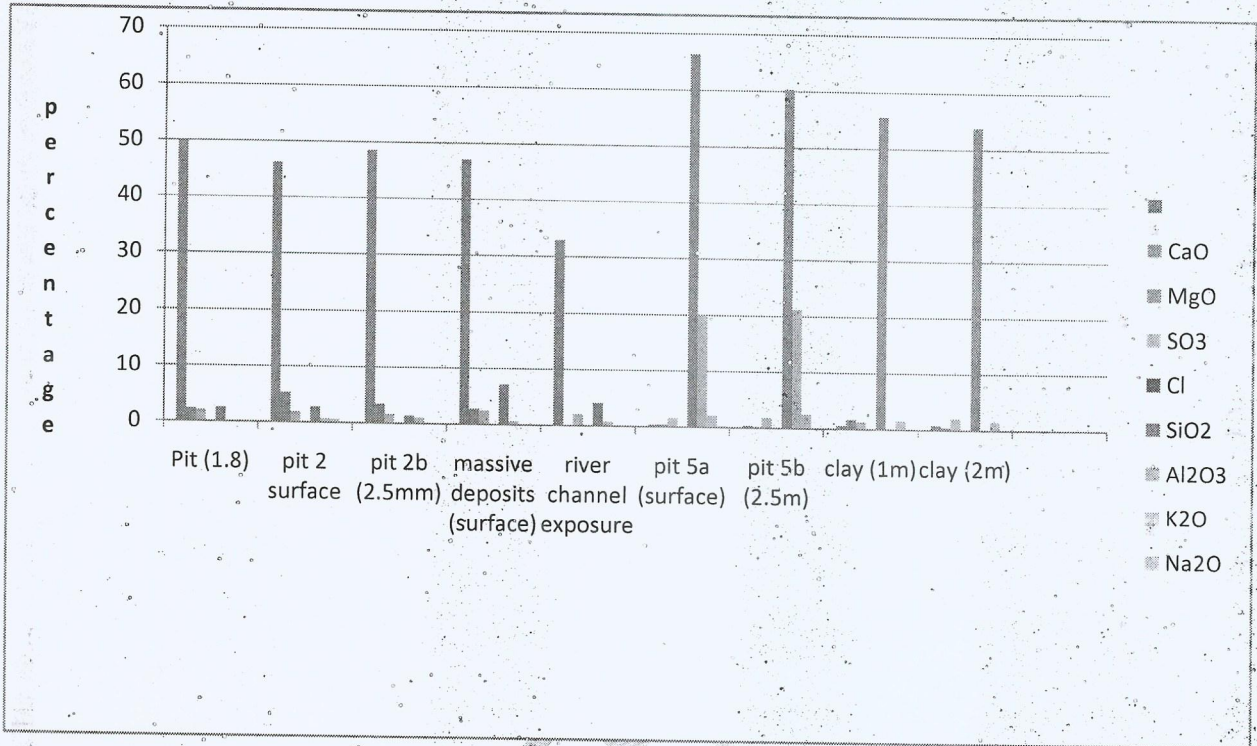
Fig. 1, Chemical composition of Itobe Limestone deposit → bold
